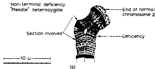
Fig. 4. (a) Salivary gland preparation of the right half of the third chromosome. The two components are united through a part of their length (above left). One component had a terminal inversion. This part conjugated with the corresponding normal chromosome by turning back on itself, as shown in the small diagram above ( to the right ). (b) Salivary gland preparation showing a part of chromosome 2; one component is "deficient". At the level of the deficiency the other component is bent outward so that above and below these level like bands meet. (After Bridges.)
